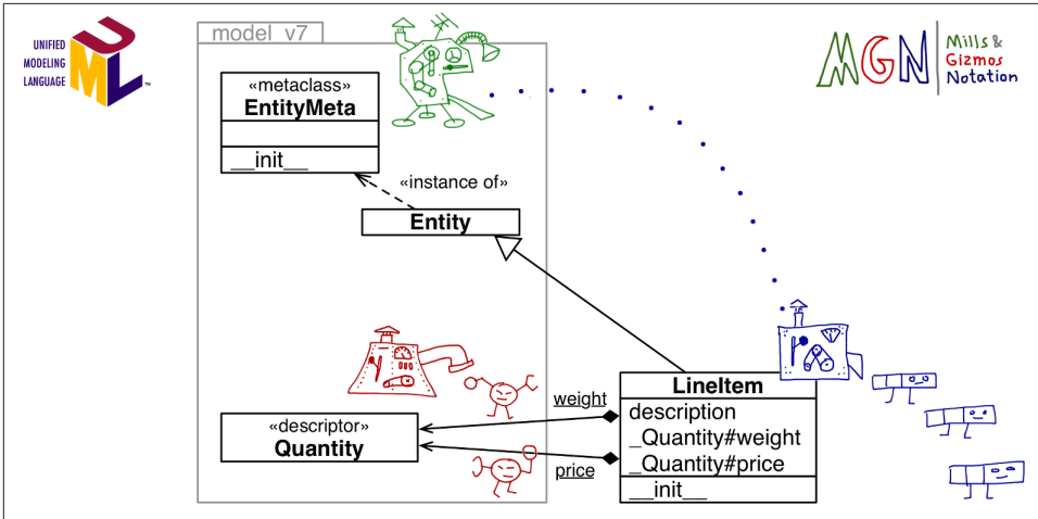
Figure 21-4. UML class diagram annotated with MGN (Mills & Gizmos Notation): the EntityMeta meta-mill builds the Lineltem mill. Configuration of the descriptors (e.g., weight and price ) is done by EntityMeta.__init__ . Note the package boundary of model_v7 .
