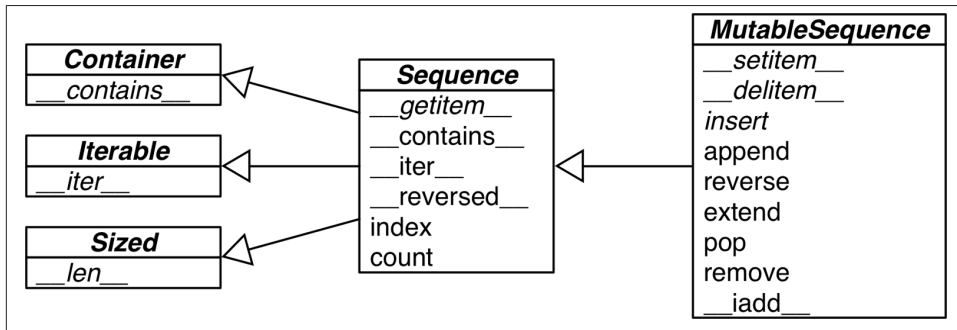
Figure 11-2. UML class diagram for the MutableSequence ABC and its superclasses from collections.abc (inheritance arrows point from subclasses to ancestors; names in italics are abstract classes and abstract methods)
